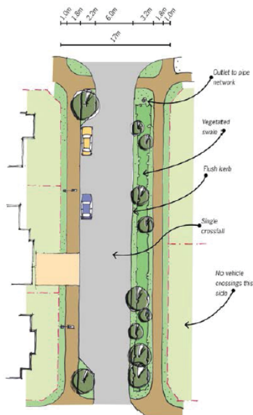
Figure 20 - Planting Guide - Swale Road - Stage 2
